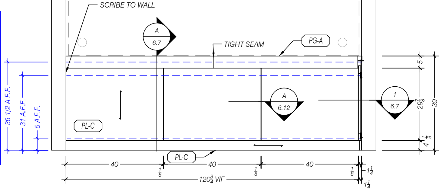
2 ELEVATION NORTH - BREAK ROOM 115 SCALE 1:24 (1/2"=1'-0") ARCH REF: 2/AE407
